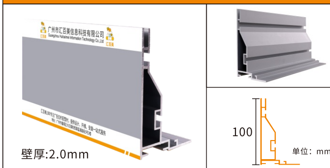
HBMC-100卡布铝型材
