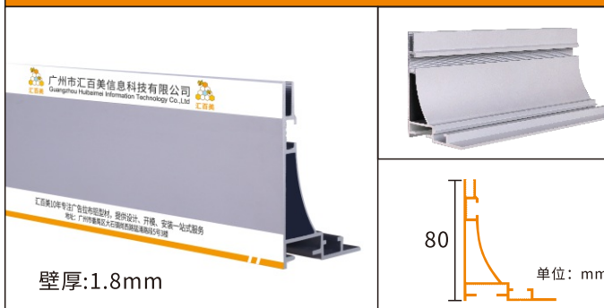
HBMC-80卡布铝型材
