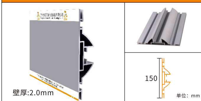
HBMCD-150双面卡布铝型材
